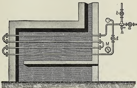
FIG. 7.—Steam Superheater.
